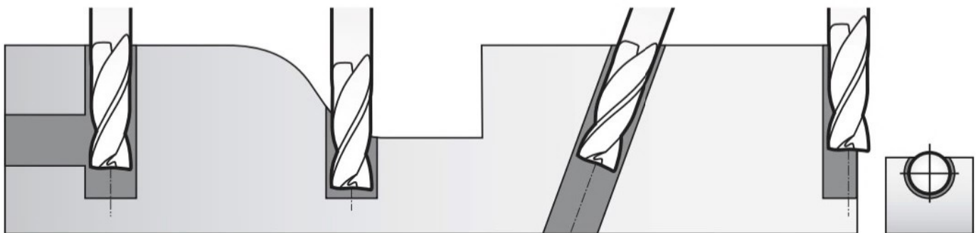
Burr-Free Intersecting Holes Shoulder Drilling Drilling Angled Holes Creating a Guide Hole
